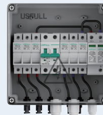
COMPACT ABS PV COMBINER BOX
