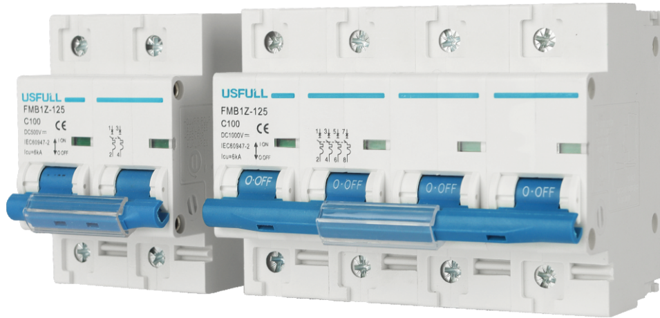
FMB1Z-125 DC Breaker (DC MCB)
