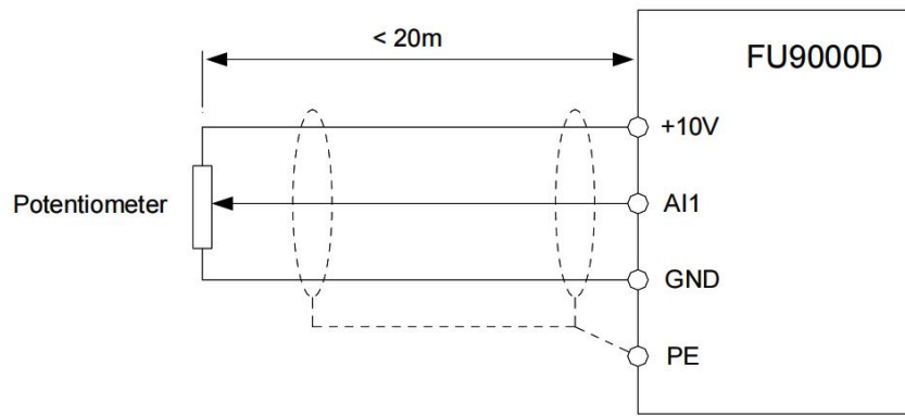
Figure 2-6 Wiring Mode of AI Terminals
